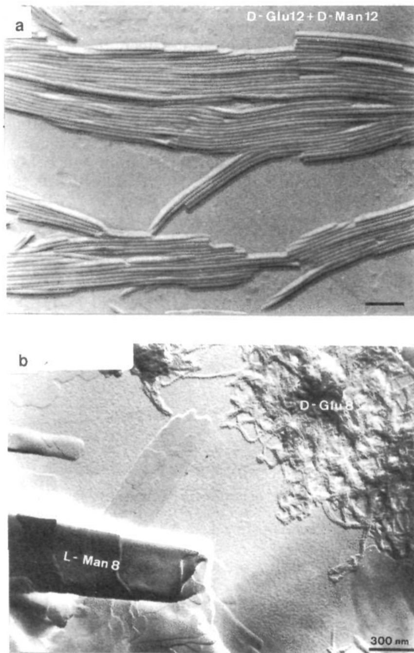
Figure 17. (a) D-Configured, diastereomeric glucon- and mannonamides form uniform tubules ("alloys"), whereas (b) an analogous 1:1 mixture of D-glucon- and L-mannonamide separate quantitatively into scrolls and helical rods. 47
