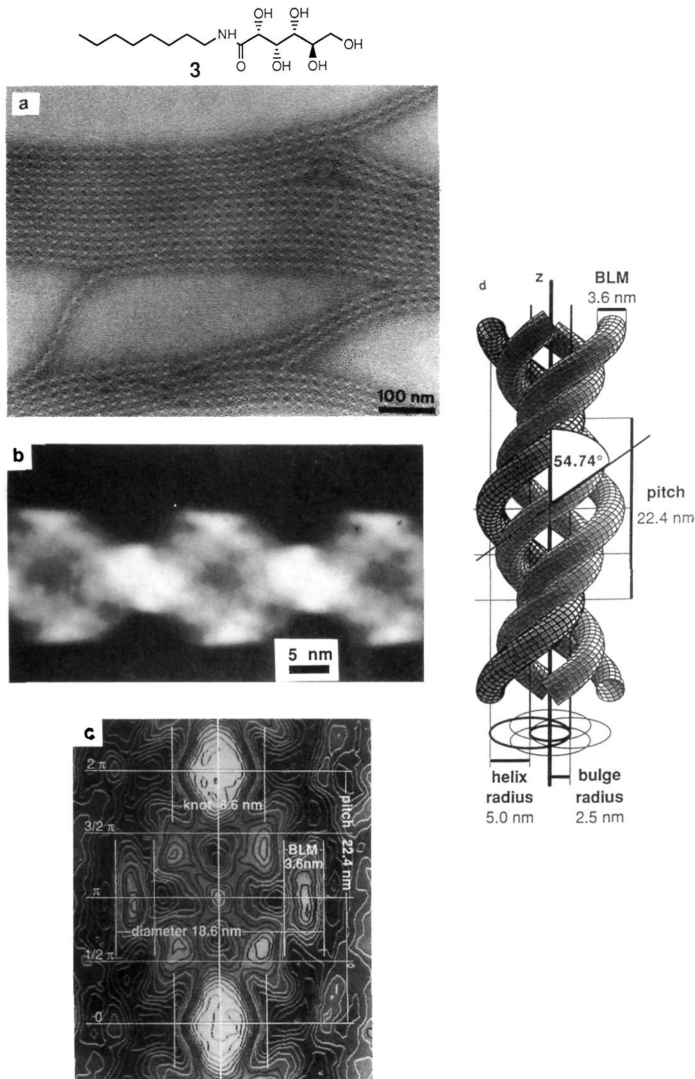
Figure 5. A well-defined molecular bilayer assembly in form of a quadruple helix has been obtained from N -octyl-D-gluconamide ( 3 ): 21 (a) electron micrograph of a fiber bundle; (b) magnification of a; the diameter of the white knots is 7.4 nm; (c) contour line diagram obtained by image analysis; (d) computer model of the fiber.
