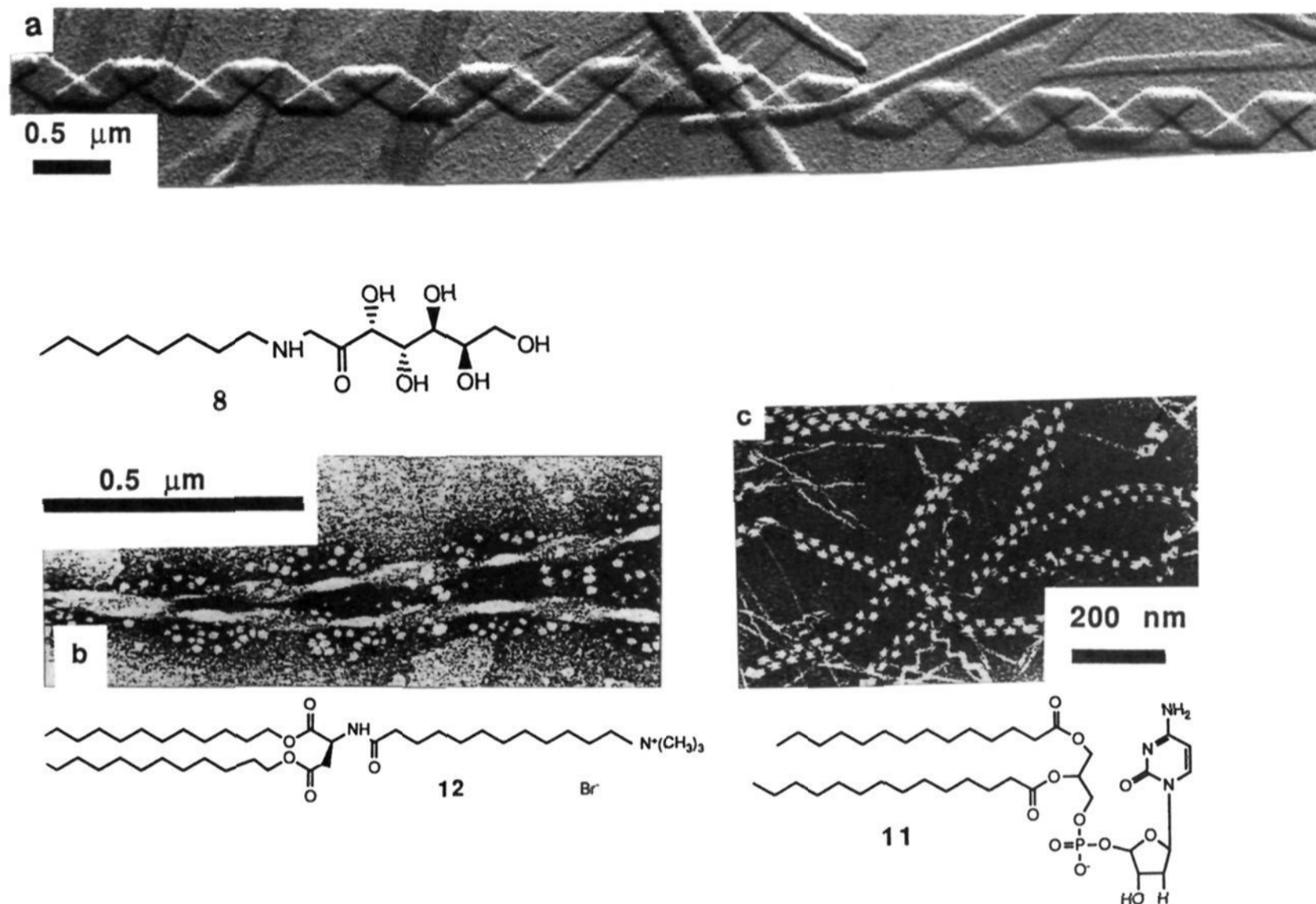
Figure 11. Electron micrographs of helical ribbons made of (a) N -octyl-D-galactonamide (8), (b) a double-chain glutamic ester with a tetraalkylammonium head group 12 34 (by kind permission of Prof. T. Kunitake), and (c) a double-chain phospholipid with a nucleotide head group 11 33 (by kind permission of Prof. H. Yanagawa). All three amphiphiles also form tubules.
