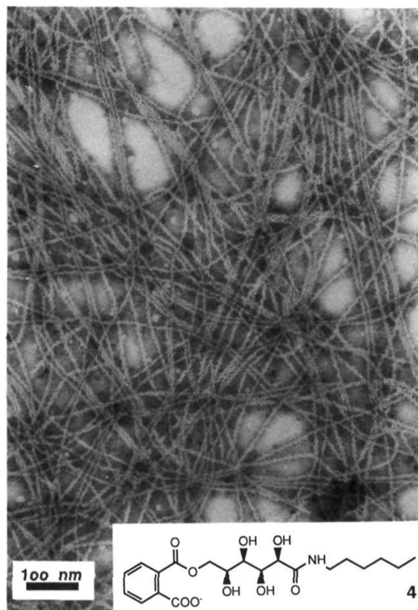
Figure 6. The micellar fibers made of the anionic gluconamide 4 (width 4–5 nm) can be packed very tightly. No merging occurs. Reference 23.
